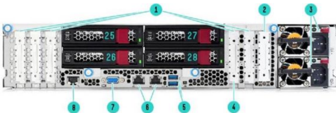
HPE StoreEasy 1650 Expanded Storage - Rear view
